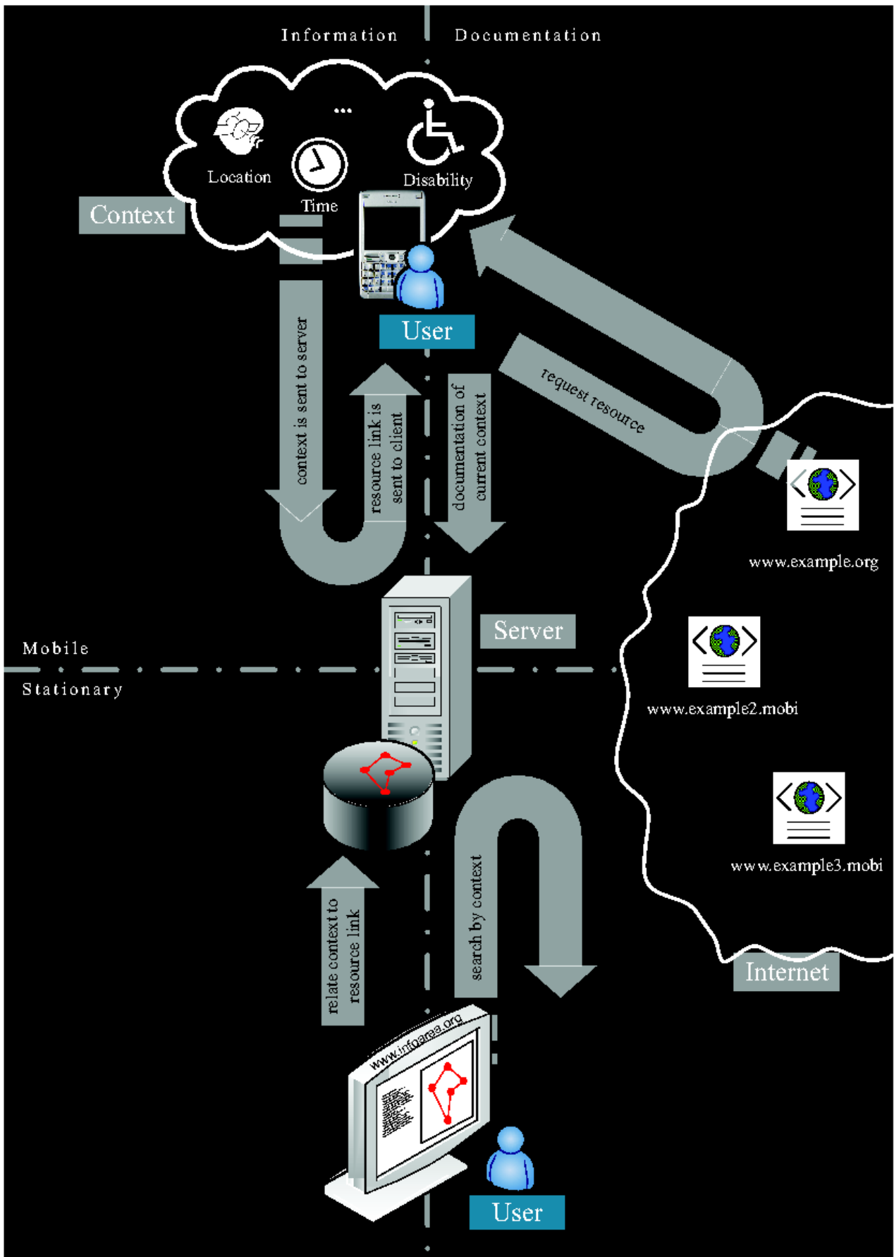
Figure 3: InfoArea system components and information flows
